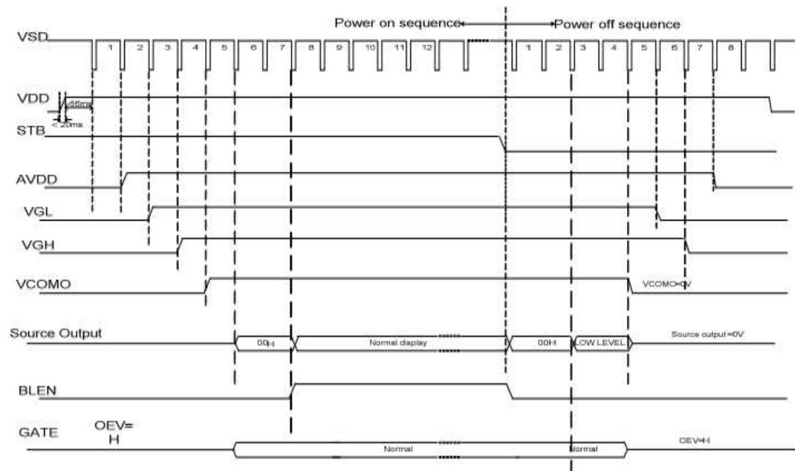
Power On/Off timing chart
