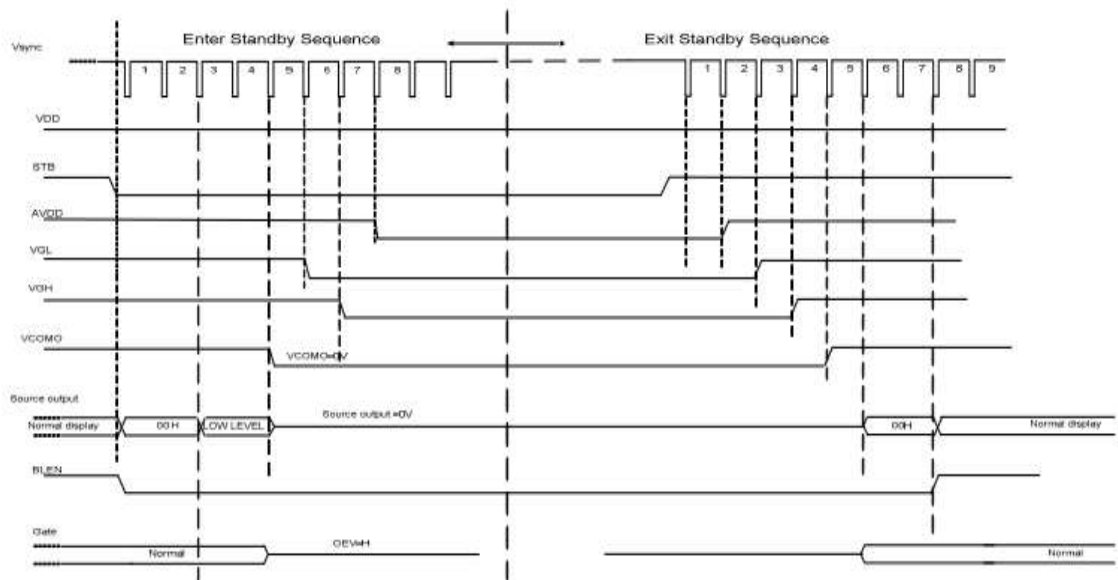
Enter and Exit Standby Mode timing chart
